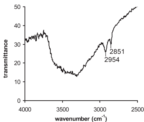
Figure 2. The FTIR spectrum of functionalized porous glass 1 , in which the \text{C-H}_x stretching modes observed at 2851 and 2954\text{ cm}^{-1} were assigned to saturated carbons of the spacer methylene groups indicating that 12 and (\text{CH}_3\text{O})_3\text{SiCH}_2\text{CH}_2\text{CH}_2\text{I} (1:3 ratio) were anchored to the PVG surface. The FTIR spectrum of a clean piece of PVG was not identical, no \text{C-H}_x stretching modes were observed.
