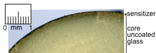
Figure 3. A low-magnification ( 10\times ) cross-sectional optical image. The dark green thin coating shows the depth of 1 accessed into PVG. The image shows \sim 0.08\text{ mm} penetration depth on the outer face of the cylinder-shaped PVG cap 1 (diameter 5.0\text{ mm} \times length 8.0\text{ mm} ).
